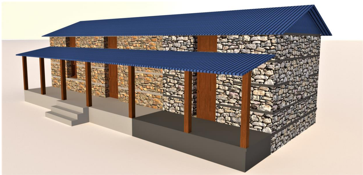
Figure 23. Addition of a room at one of the widths with the provision of buttresses in case of stone in mud building
