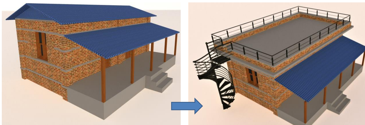
Figure 29. Showing the transformation of the building after replacing light roof with RC roof
