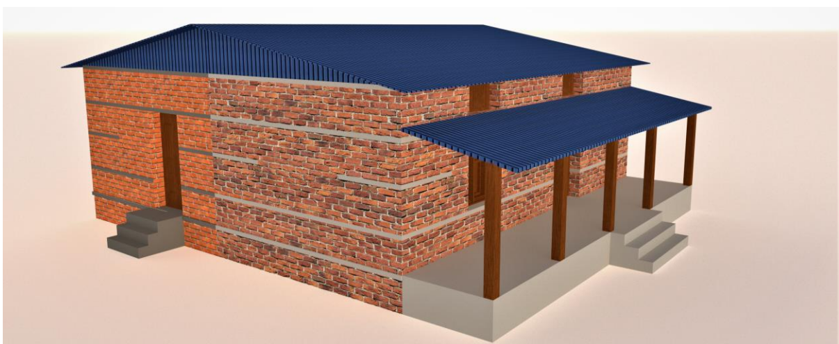
Figure 26. Addition of two rooms at one of the lengths with the provision of buttresses in case of brick in cement building
