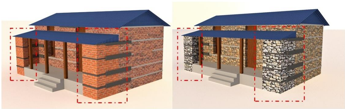
Figure 6. Addition of wing walls in same direction
