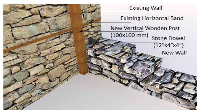
Figure 11. Stone dowels connecting the existing wall and the new wall in case of wooden reinforcement
