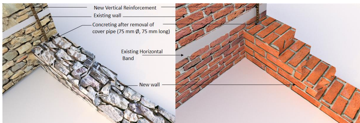
Figure 8. 3D depicting the placement of a new vertical rebar in stone masonry (left) and brick masonry (right) walls
