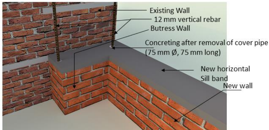
Figure 22. Provision of buttress to stiffen the new wall where cement and reinforcement are available in case of brick masonry
