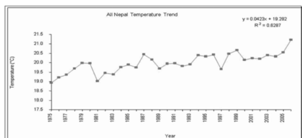
Figure 1.4: All Nepal temperature trend (1975-2006) Source: DHM
