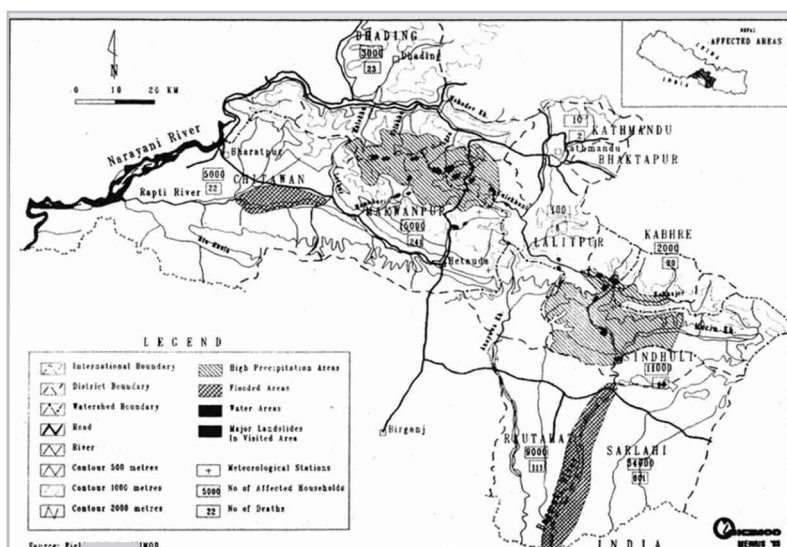
Figure 3.6: Area affected by landslides and flood disasters during high intensity rainfall of July 19 -20, 1993 Source: Dhital et al. 1993
